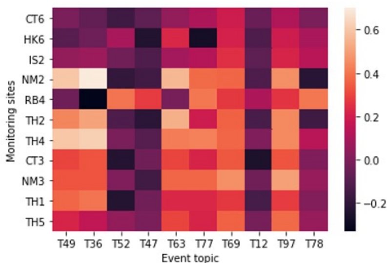
Fig. 5 Monitoring site pollutant – detected event correlation
